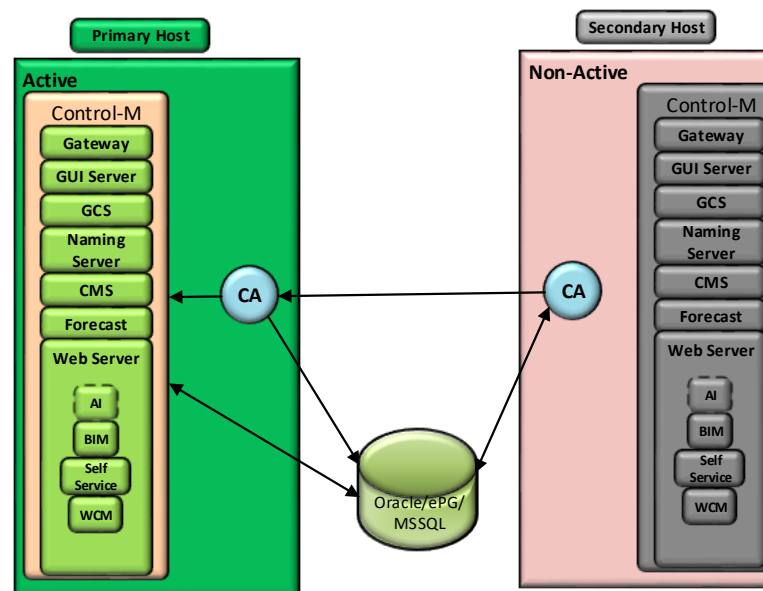
Figure 4: Control-M/EM with Oracle/MSSQL/exiting PG
