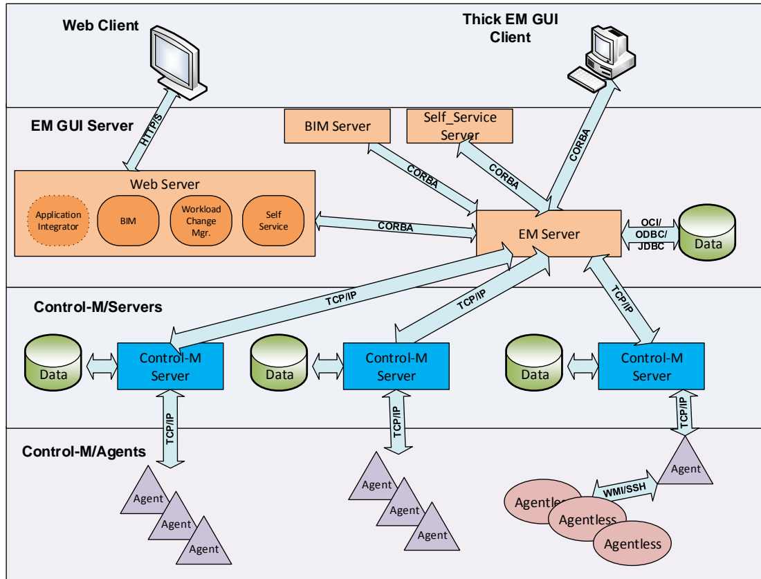
Figure 1: Basic BMC Control-M Architecture
