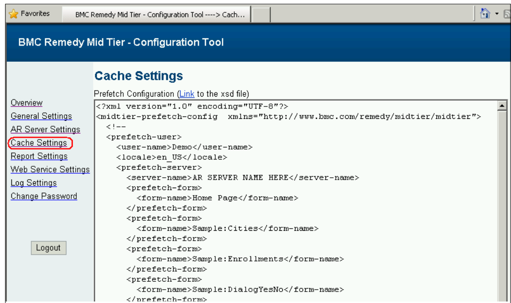
Figure 9: prefetchConfig.xml
